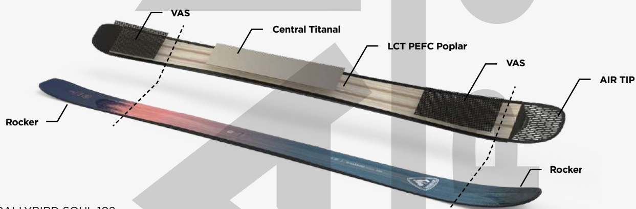
RALLYBIRD SOUL 102
